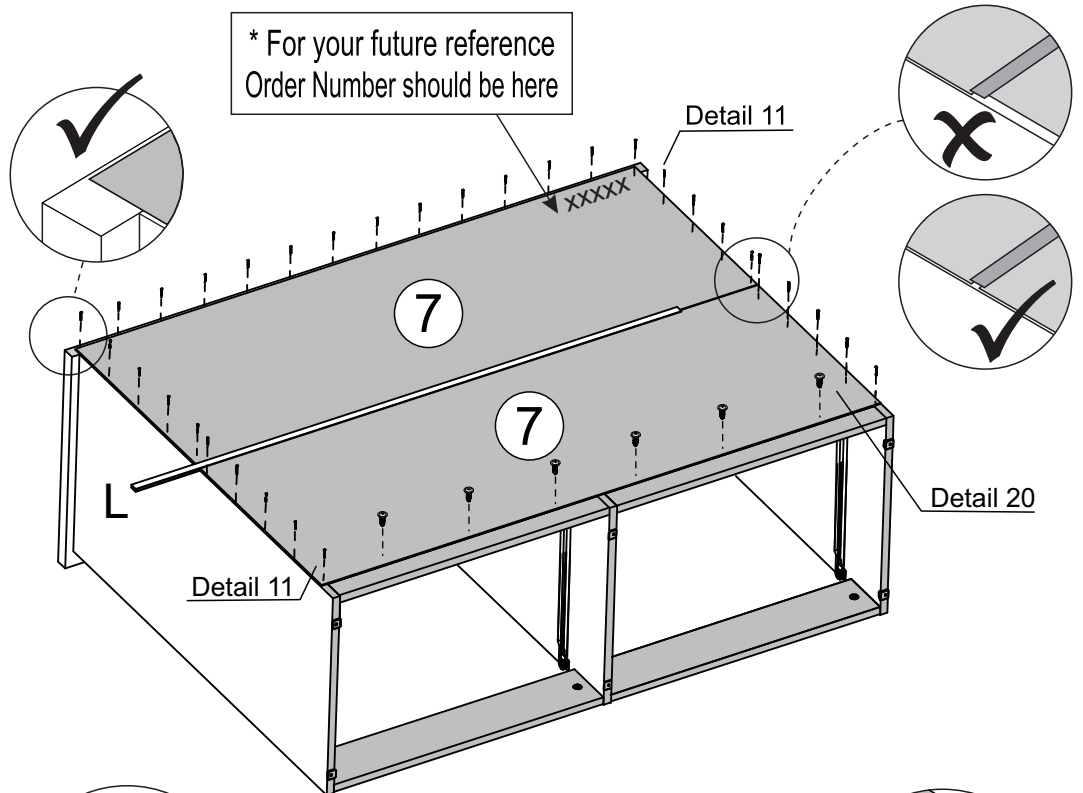
Cam bolt head needs to be in centre
