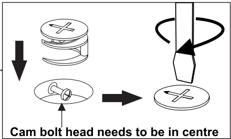
Cam bolt head needs to be in centre
