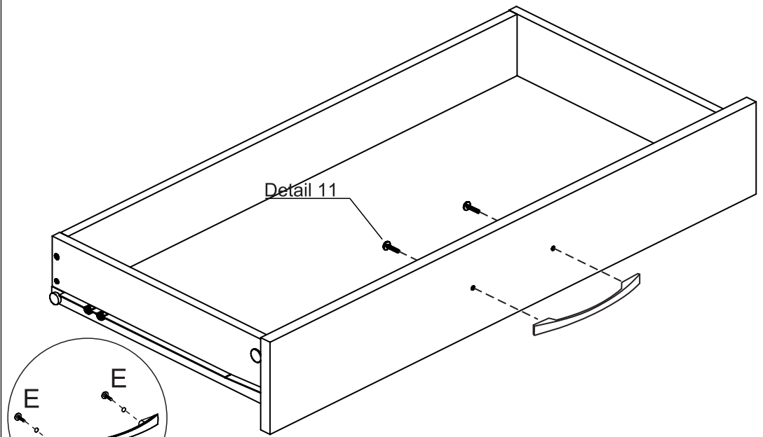
Detail 11
