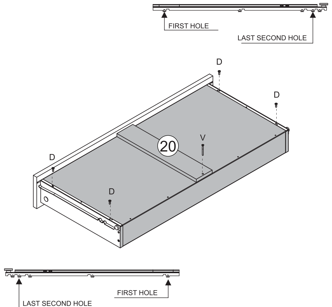
Detail 1
