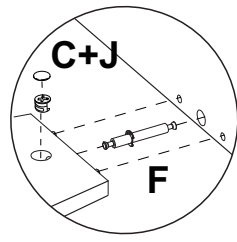
Detail 5
